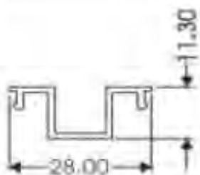
Louvre Adaptor Oval Louvre (SO*)
