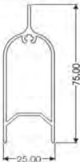
Louvre Rounded 75mm (SO*)
