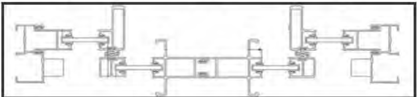
LOCK STILE - FEMALE SASH
