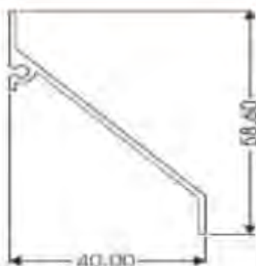
Louvre Lazy Z One Screw Port (SO*)
