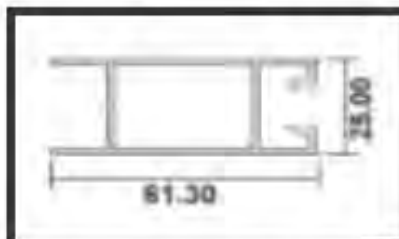
LOCK STILE - FEMALE SASH
